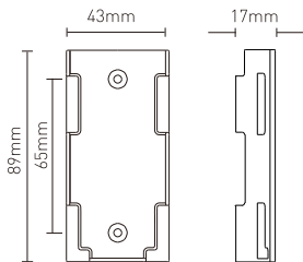
Holder
