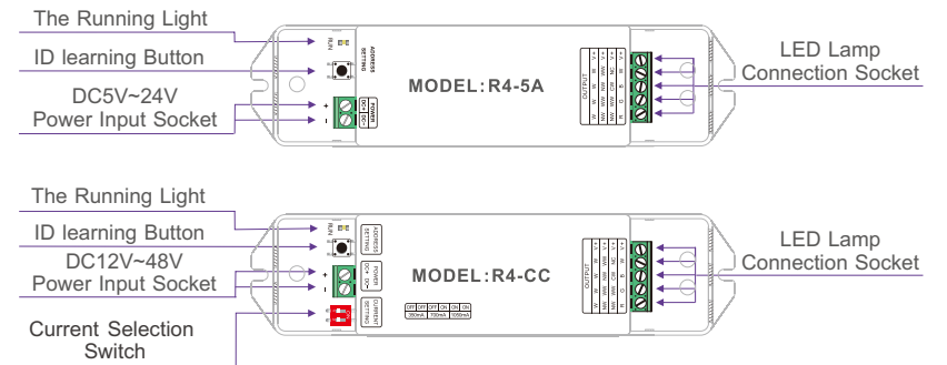
(Operation Table)
