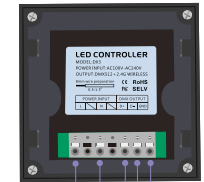
AC100-240V Power Input Socket DMX Signal Output Socket
